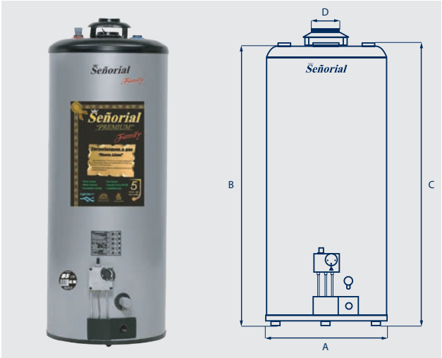
Termotanque Gris a Gas 85 Lts.
